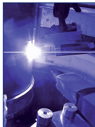
In-situ studies of welding on C2, the powder diffractometer.
